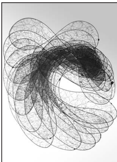
Algoritihm#01
